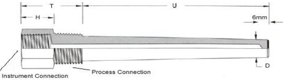
Screwed Taper Thermowell
